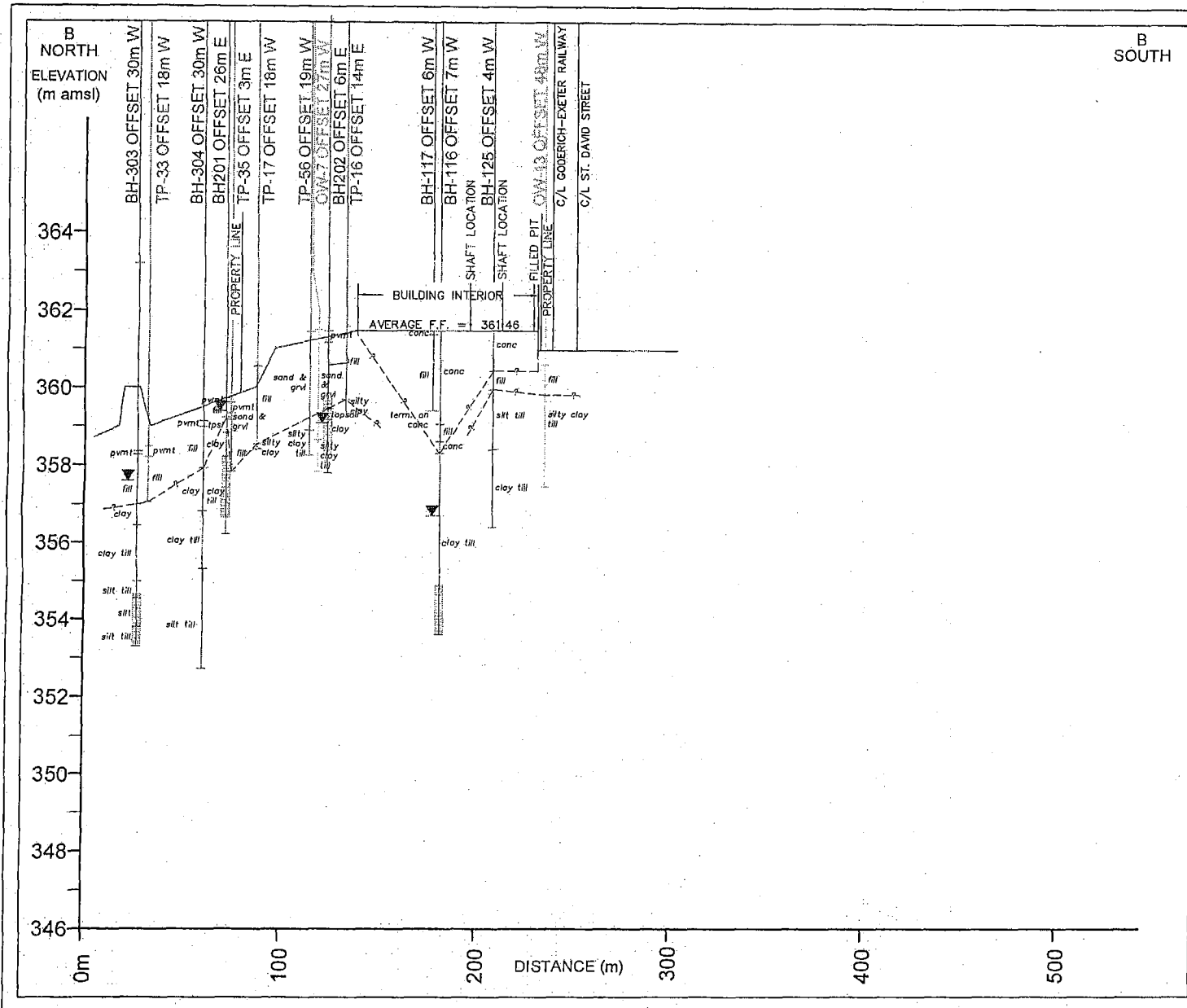
FIGURE 3 CITY OF STRATFORD COOPER SITE PROPERTY SITE CONDITIONS - MAY 2009 CROSS SECTION B-B
